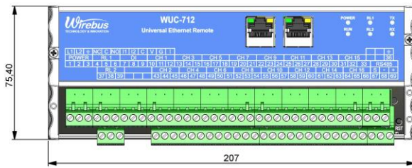
VISTA FRONTAL
