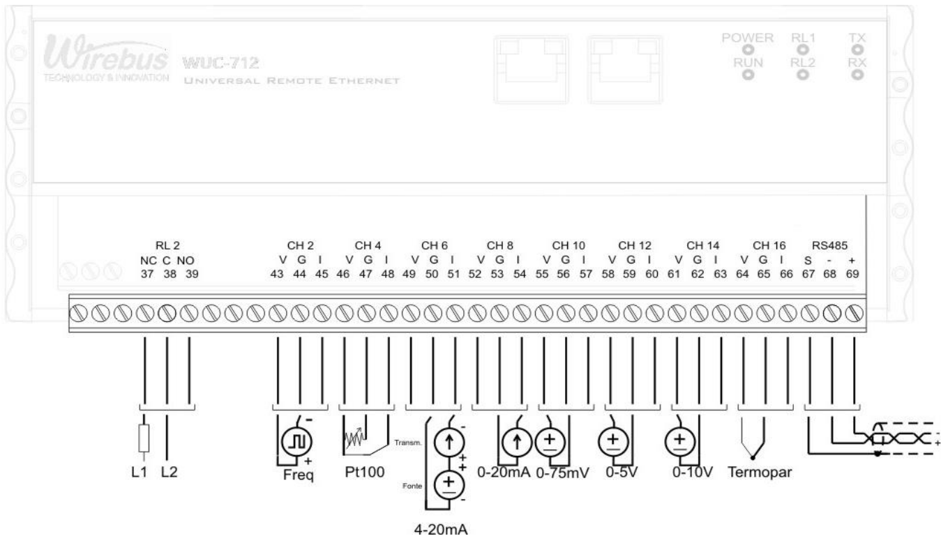
Borneira inferior
