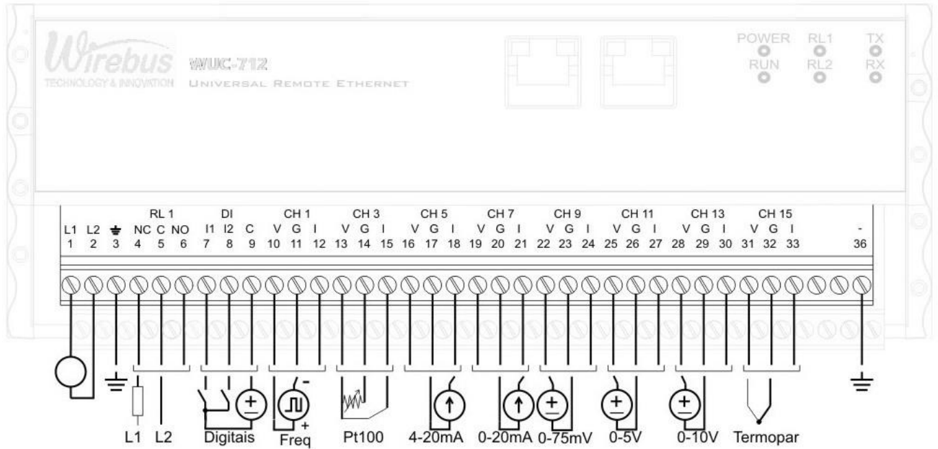
Borneira superior
