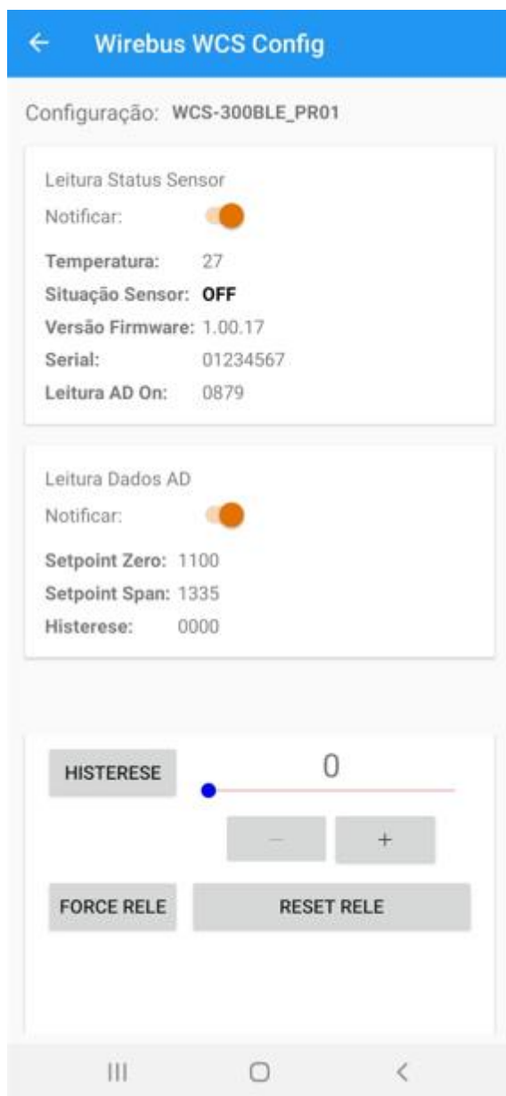
Figura 16 – Force/Reset Rele
